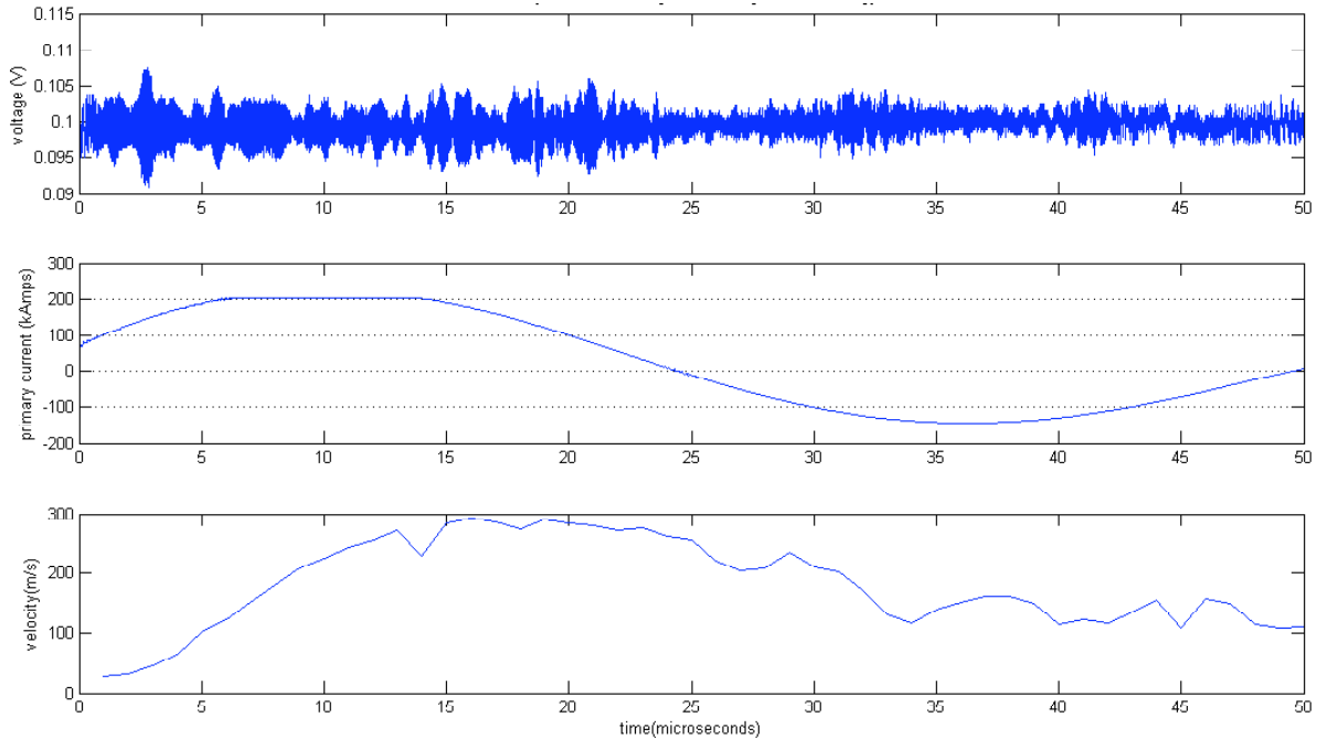
Figure 7. Primary current and impact velocity profile on magnetic pulse linear seam welding system. The launch energy is 4.8kJ and the stand off distance is 5.7mm.
